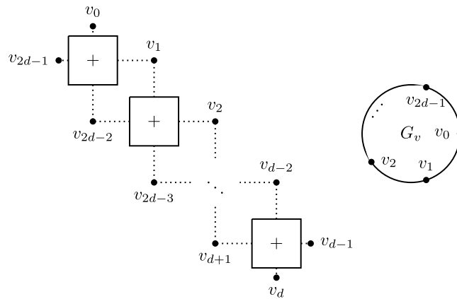
Fig. 8. Vertex gadget G_v (dotted links mean identification of vertices) and its schematic representation.
