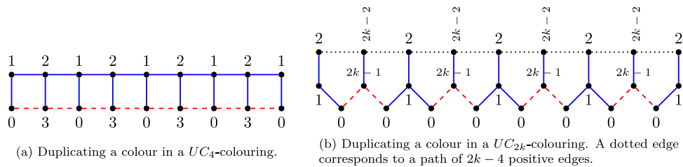
Fig. 10. Gadgets with vertices of degree 3 or 2, that are mapped to the same vertex in a UC_{2k} -colouring.
