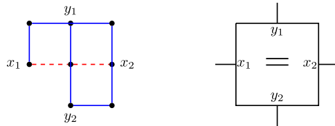
Fig. 4. Copy gadget and its schematic representation.
