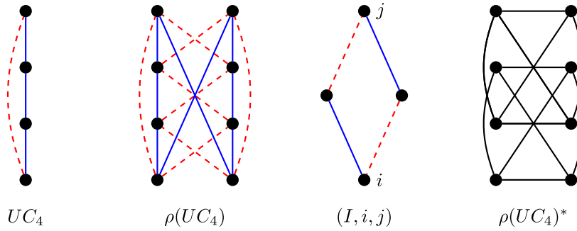
Fig. 1. The unbalanced cycle UC_4 , its switching graph \rho(UC_4) , the indicator (I, i, j) and its resulting undirected graph \rho(UC_4)^* .
