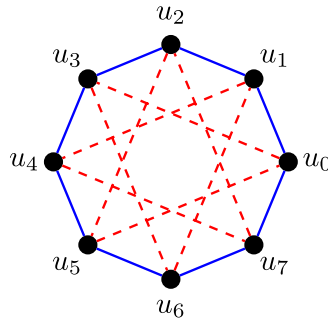
Fig. 3. The signed graph \rho(UC_4) .
