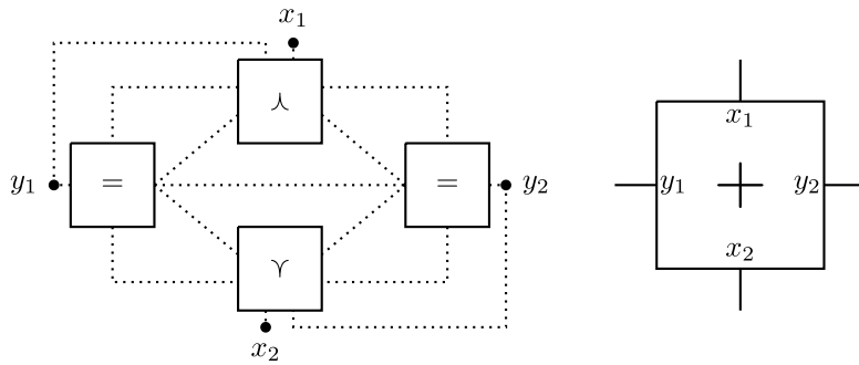
Fig. 7. Construction of the crossing gadget (dotted links mean identification of vertices) and its schematic representation.
