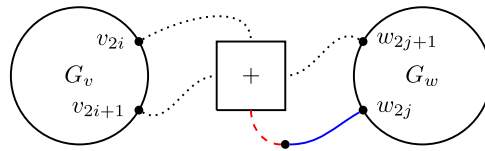
Fig. 9. Edge gadget (dotted links mean identification of vertices).
