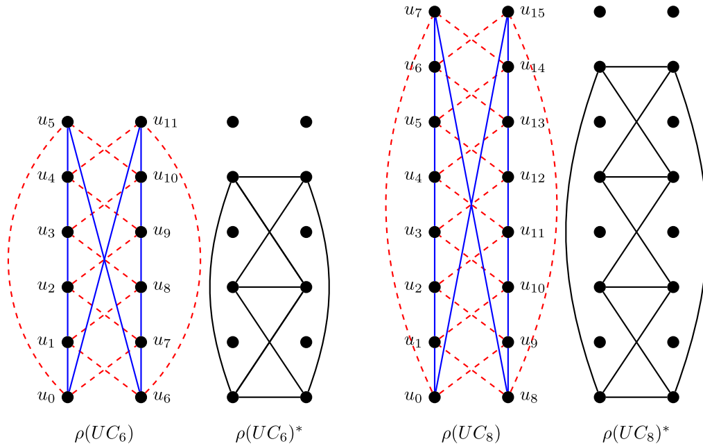
Fig. 2. The switching graphs \rho(UC_6) and \rho(UC_8) , and the undirected graphs \rho(UC_6)^* and \rho(UC_8)^* resulting from the application of the indicator (I, i, j) from Fig. 1 (in which we only draw one of the two isomorphic components). The core of \rho(UC_6)^* is K_3 and the core of \rho(UC_8)^* is K_{8/3} , the Wagner graph.
