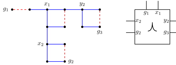
Fig. 6. Split gadget and its schematic representation.
