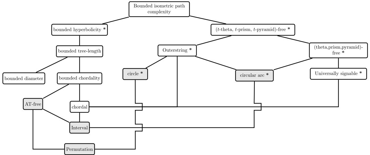
Fig. 1. Inclusion diagram for graph classes. If a class A has an upward path to class B , then A is included in B . Constant bounds for the isometric path complexity on graph classes marked with * are contributions of this paper.
