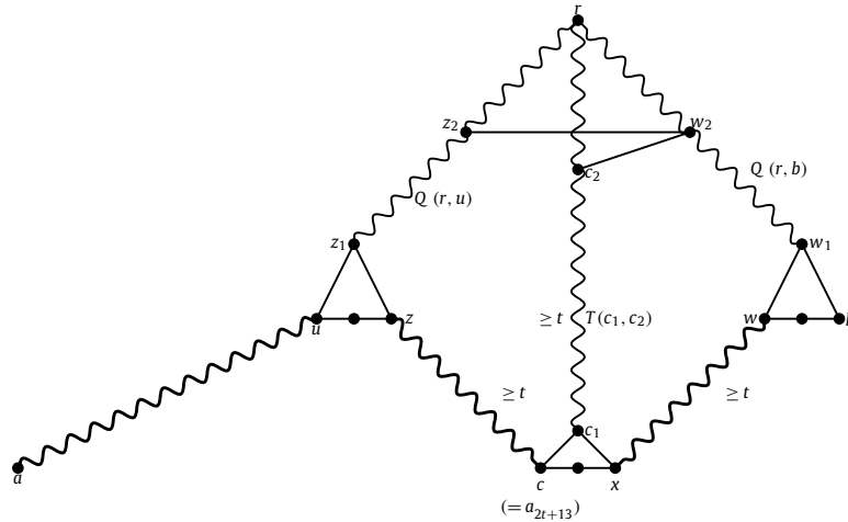
Fig. 4. Illustration of the notations used in the proof of Lemma 20. The thick wiggly line along with the horizontal edges indicate the (a, b) -isometric path P .
