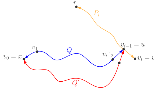
Fig. 2. An illustration for the third case in the proof of Lemma 14.
