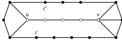
Fig. 3. An example of a 4-fat turtle. Let C be the cycle induced by the black vertices, P be the path induced by the white vertices. Then the tuple (4, C, P, c, c') defines a 4-fat turtle.
