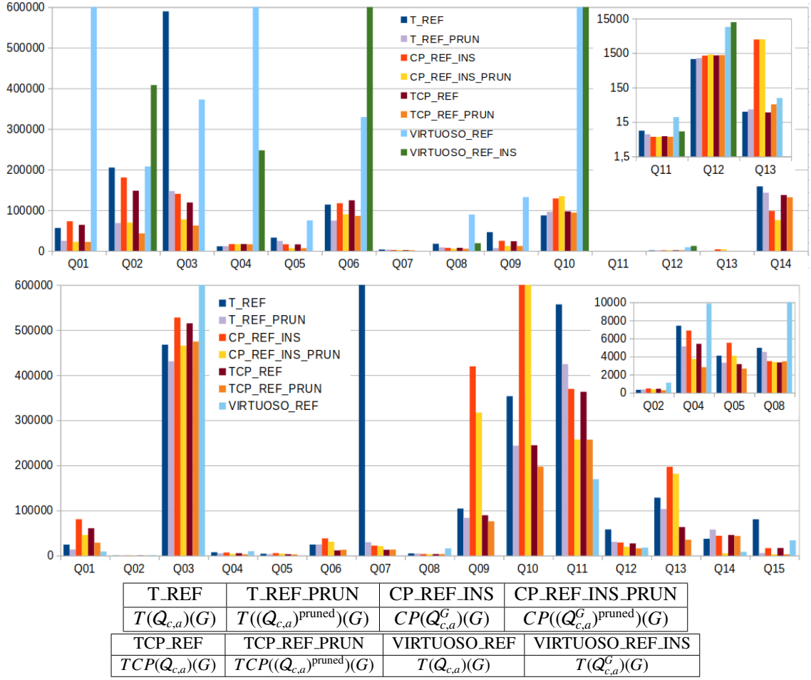
Figure 3.9: LUBM (top) and DBLP (bottom) query answering times (ms) through reformulation.
