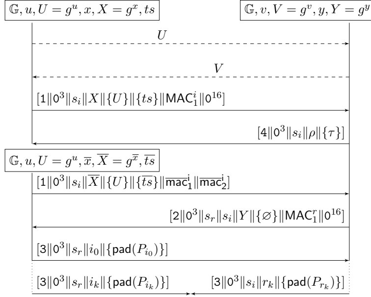
Figure 4.4: WireGuard (with cookies).
