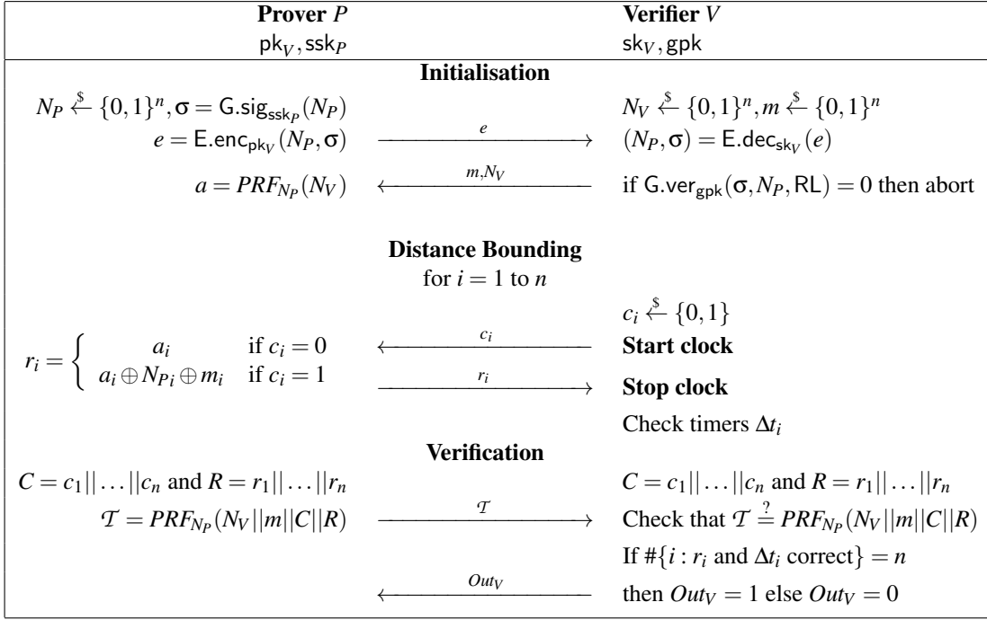
FIGURE 1: SPADE our anonymous TF resistant protocol that uses a public key encryption E = (E.\text{enc}_{pk_V}(m), E.\text{dec}_{sk_V}(c)) , a pseudo-random-function set PRF and a revocable group signature G = (G.\text{sig}_{ssk_P}(m), G.\text{ver}_{gpk}(\sigma, m, RL)) , where a||b is the concatenation of a and b ; x \xleftarrow{\$} U is random value uniformly chosen in U and x \oplus y denotes the exclusive-or.
