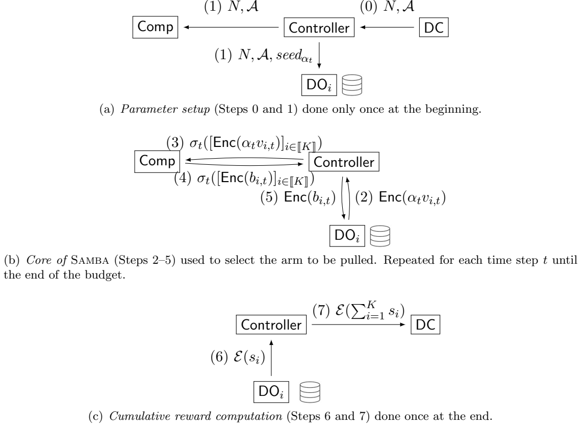
Figure 5: Architecture of SAMBA.
