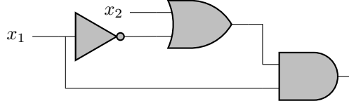
Figure 3: Circuit of our running example (\overline{x_1} \vee x_2) \wedge x_1 .
